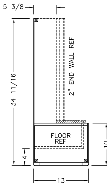
CHEST TOP VIEW
