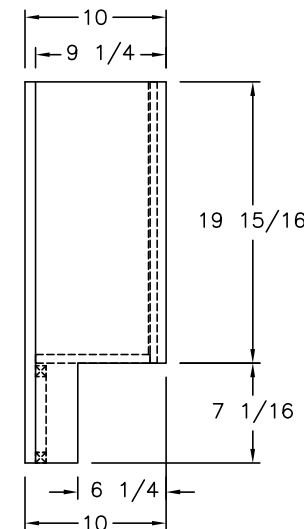
RT SIDE VIEW
