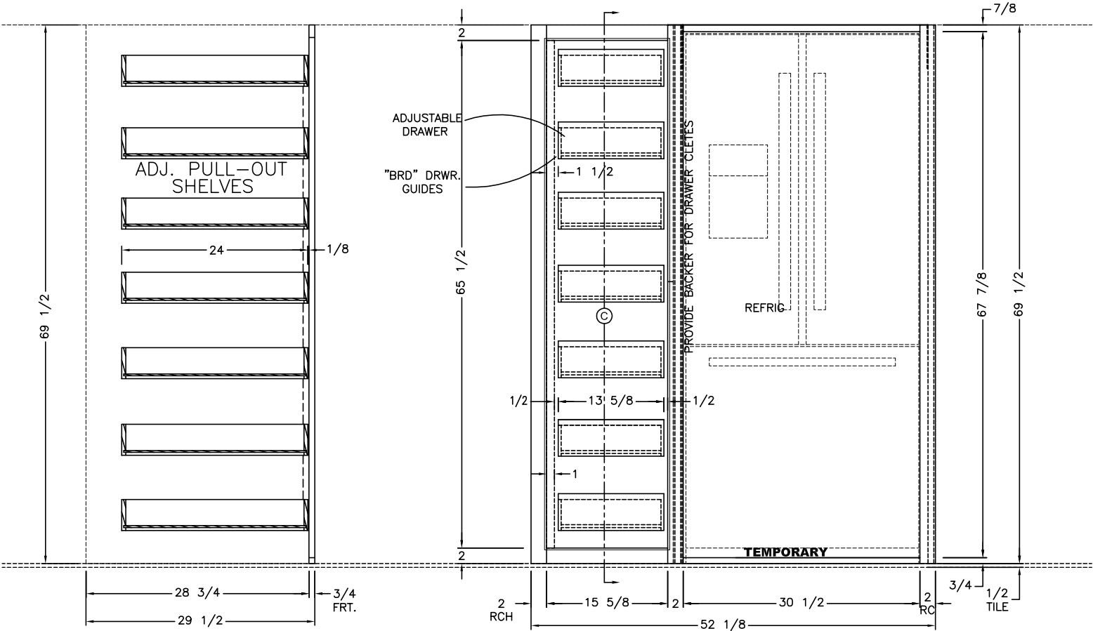
FRONT VIEW (1) 16 1/8 X 66 DOOR
