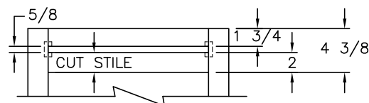
CABINET BASE FRONT VIEW
