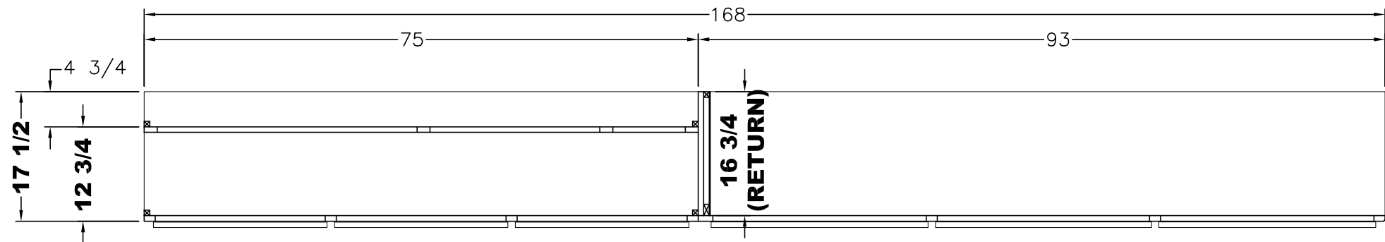
PLAN VIEW
