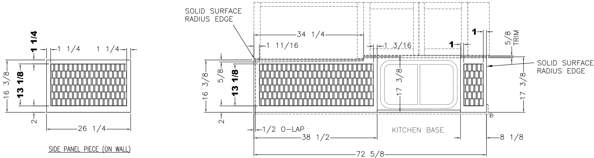
TILE/SOLID SURFACE BACKSPLASH SOLID DENOTES 1/4" RECESS FOR TILE INLAY
