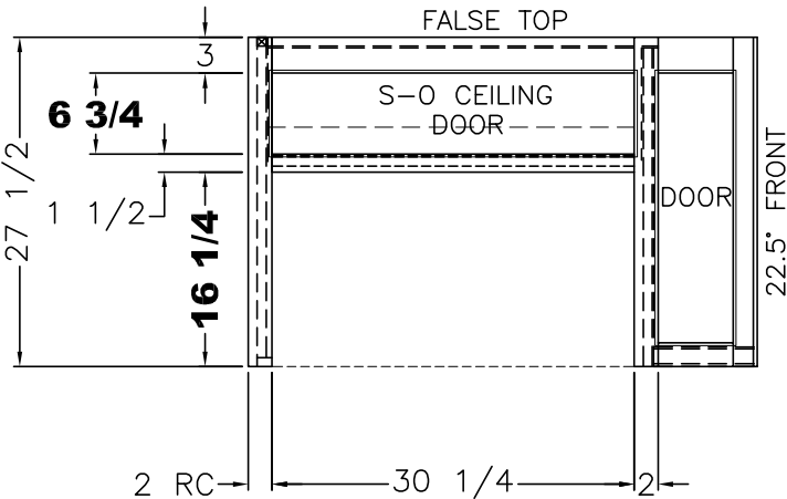
VIEW (B) (1) 7 1/4x30 3/4 HINGE DOOR (1) 6 3/4x23 1/4 DOOR
