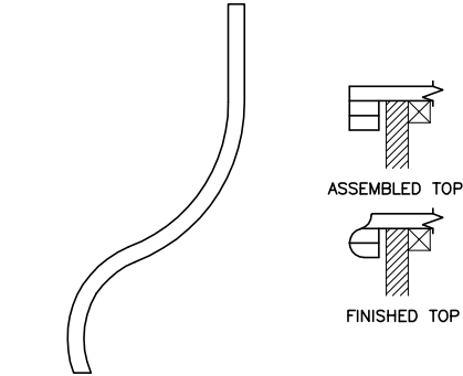
EDGE TRIM (2) PIECES 1/2 MATERIAL
