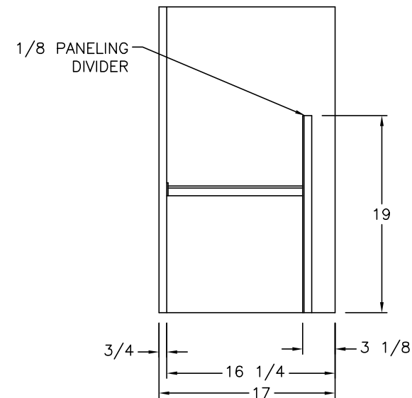
SIDE SECTION (A)
