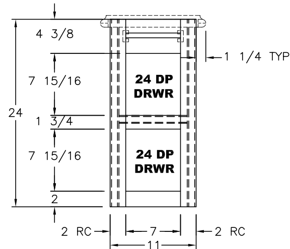
FRONT VIEW (2) 7 1/2x8 1/2 FRONTS
