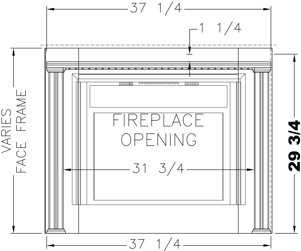
FRONT VIEW (ASSEMBLED)
