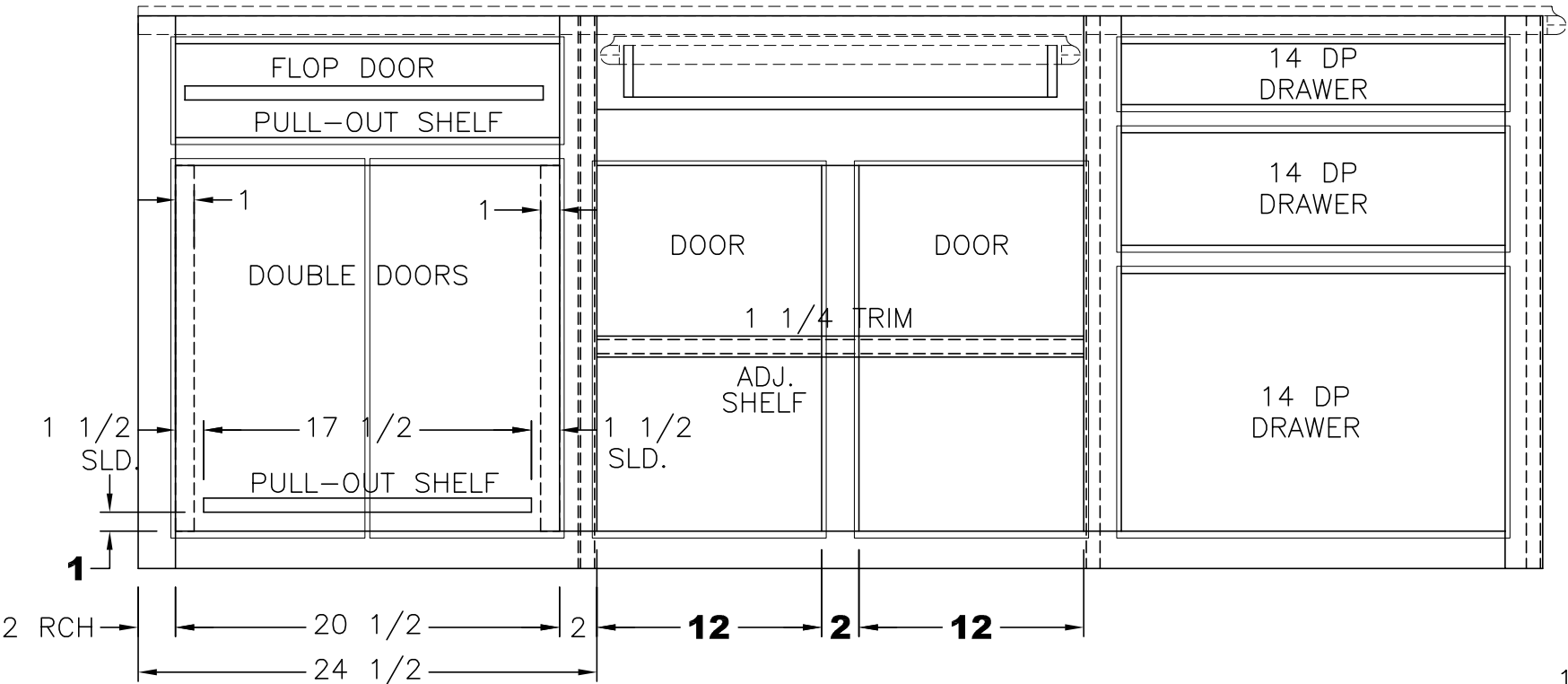
(2) 12 1/2x20 1/8 DOORS (HINGE DOORS ON CENTER STILE)
