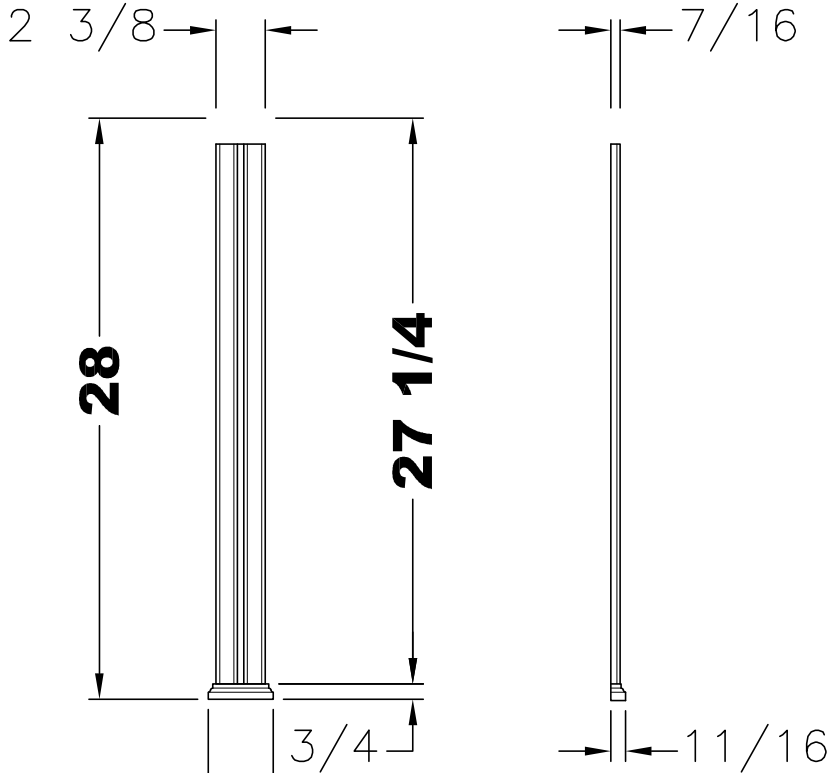
COLUMN DETAILS
