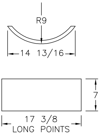
FRONT COVER LAID OUT FLAT
