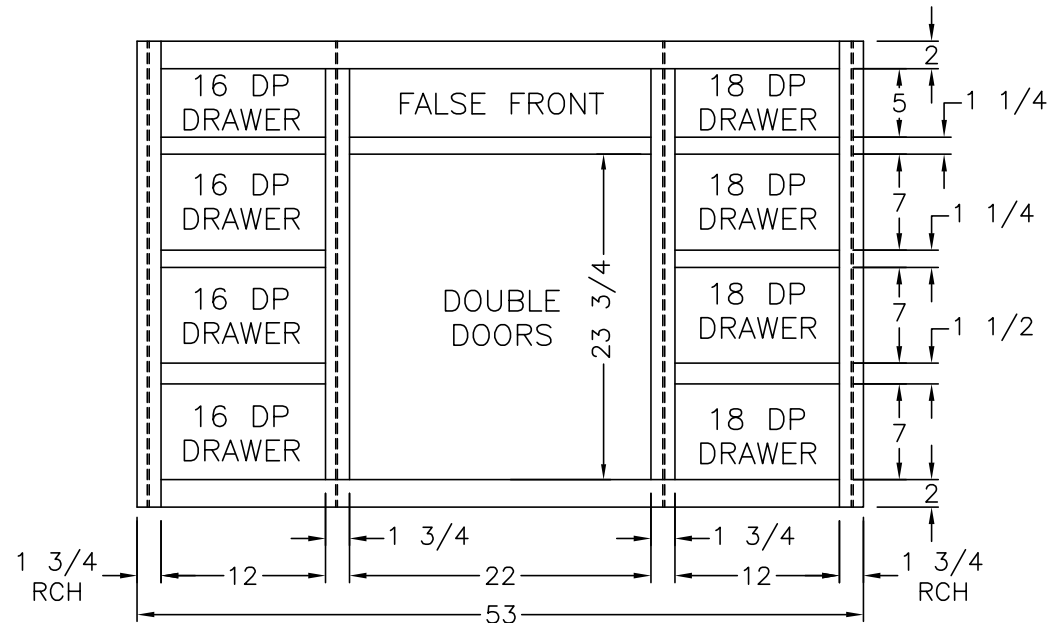
(2) 5 1/2x12 1/2 DRAWER FRONTS (6) 7 1/2x12 1/2 DRAWER FRONTS (2) 11 1/8x24 1/4 DOORS (1) 5 1/2x22 1/2 FALSE FRONT
