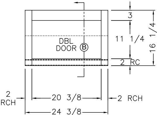
FRONT VIEW (C) (2) 10 3/8 X 11 3/4 DOORS
