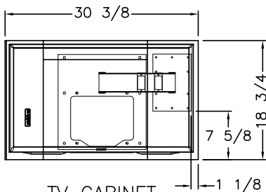
TV CABINET
