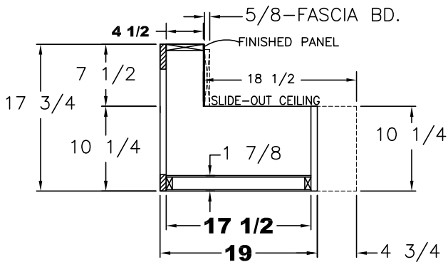
SIDE SECTION Ⓐ
