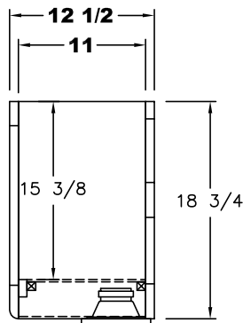
SECTION F-F
