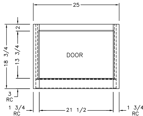
FRONT VIEW VIEW B (1) 22 x 14 1/4 DOOR
