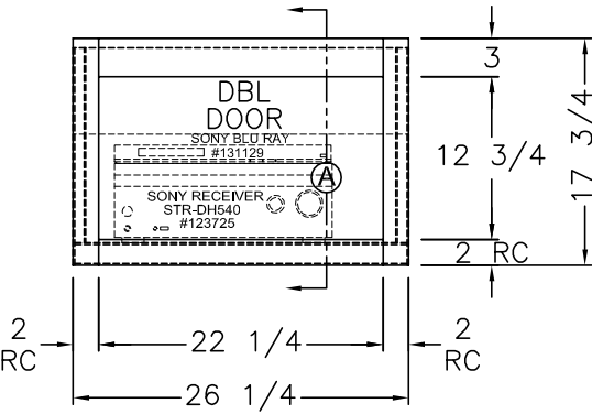
FRONT VIEW (B) (2) 11 1/4 X 13 1/4 DOORS
