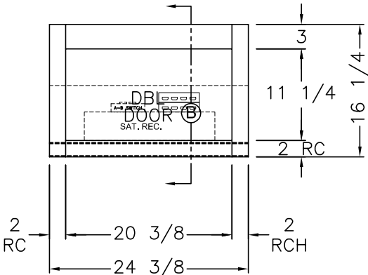
FRONT VIEW (A) (2) 10 3/8 X 11 3/4 DOORS
