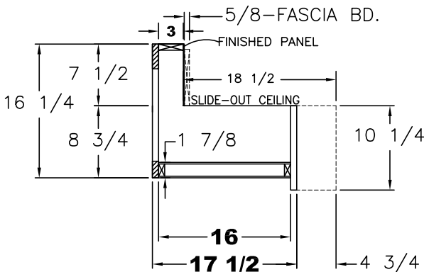
SIDE SECTION Ⓑ
