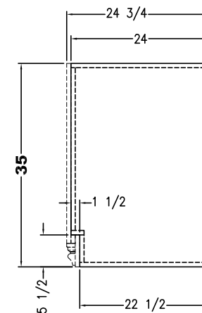
REAR END PANEL
