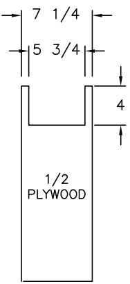
BACK PANEL DETAIL
