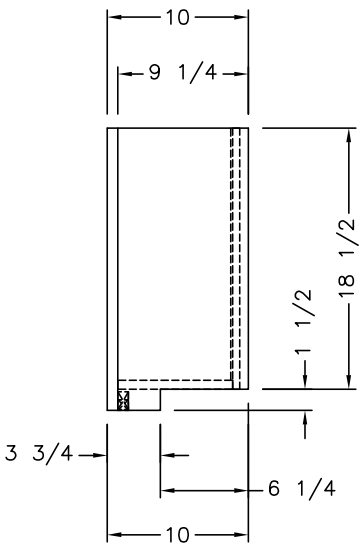
RT SIDE VIEW
