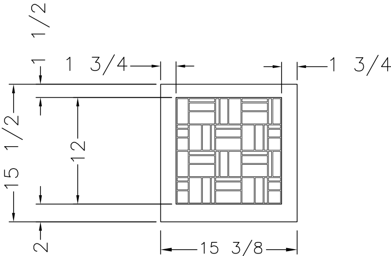
VIEW A
