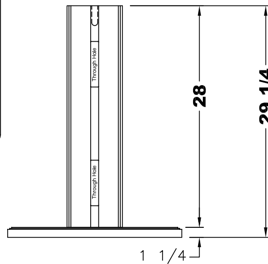
FREE STANDING LEG FOR TABLE
