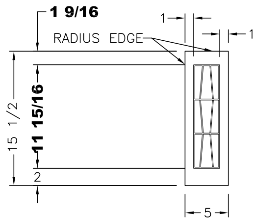
VIEW A
