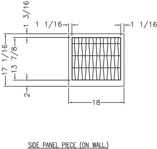
TILE/SOLID SURFACE BACKSPLASH (T360) KITCHEN WINDOW
