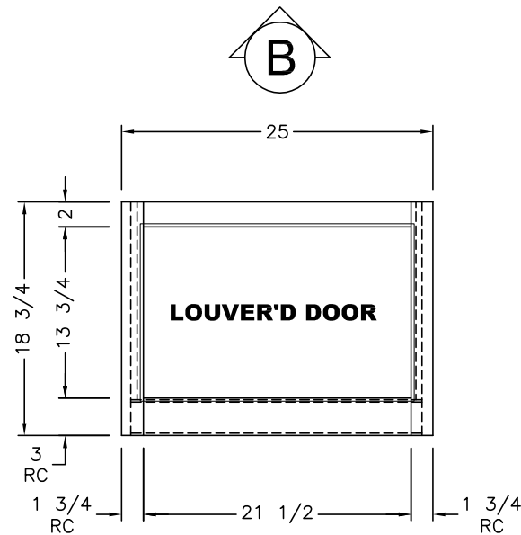
FRONT VIEW VIEW B
