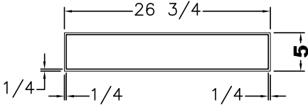
DOOR OVERLAY (1) 5x26 3/4 FRONT
