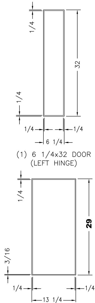
(1) 13 1/4x29 DOOR (LEFT HINGE)
