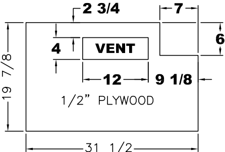
DETAIL 'F'
