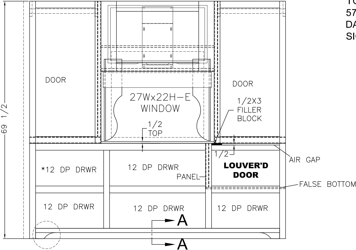
FRONT VIEW (1) 11x20 3/8 LOUVER'D DOOR (BOTTOM HINGE)
