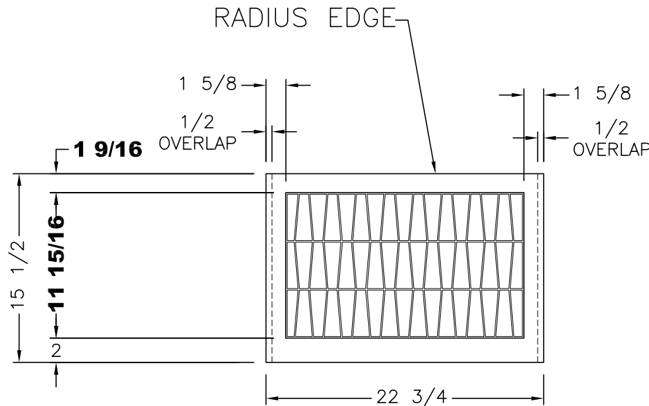
VIEW B
