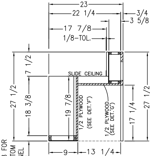
SIDE SECTION (G)
