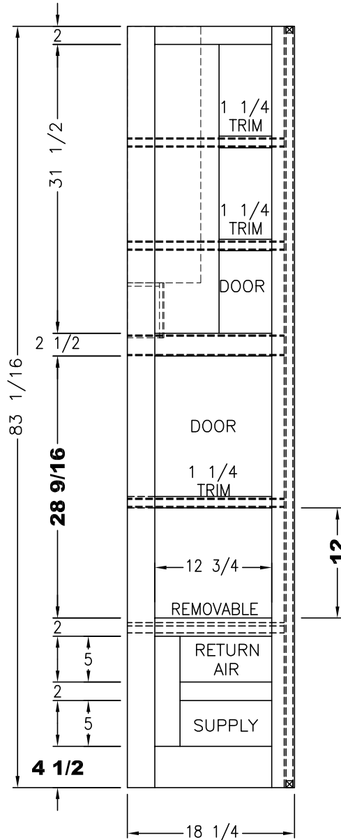
VIEW (A)
