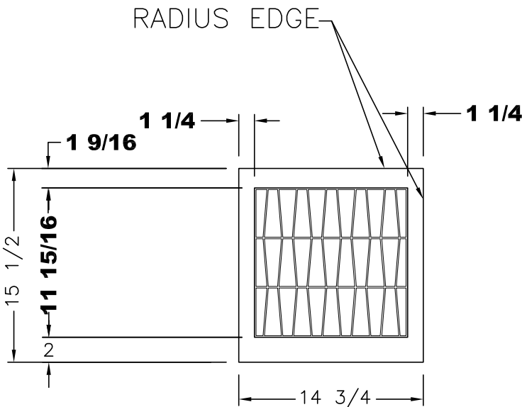
VIEW C
