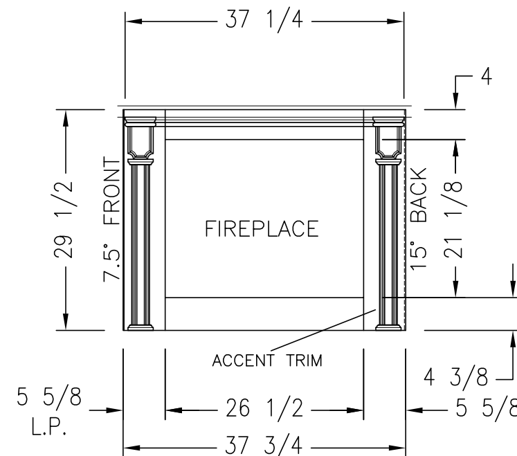
FRONT VIEW (B)
