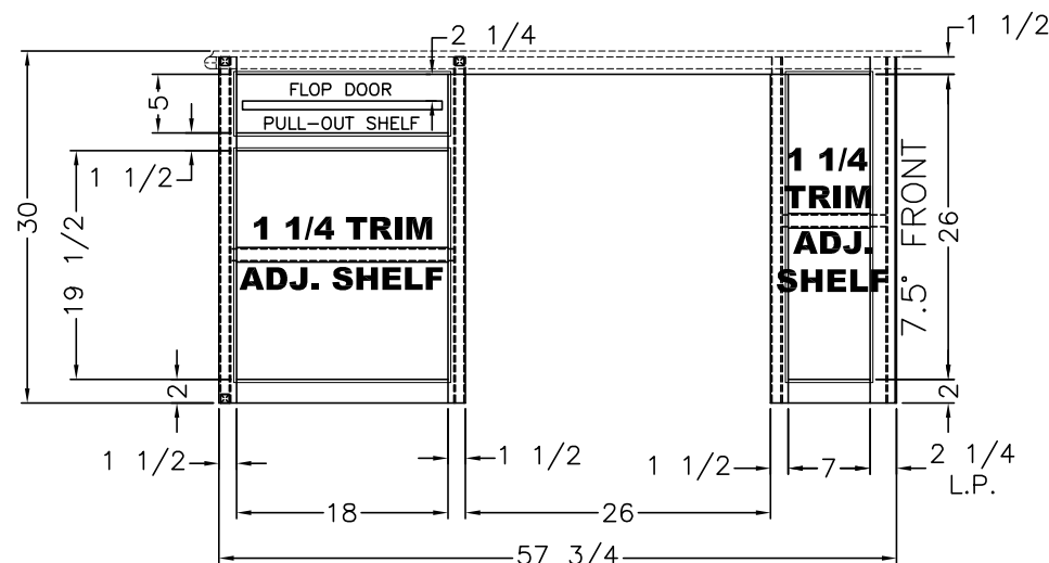
FRONT VIEW (A)
