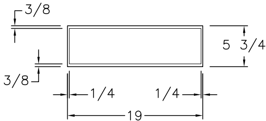
(2) 5 3/4 x 19 FRONT
