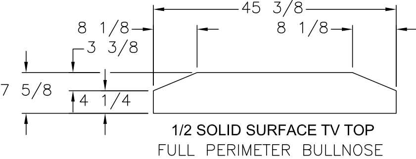
1/2" SOLID SURFACE CABINET TOP ▶ - DENOTES A FINISHED EDGE * - PENCIL EDGE
