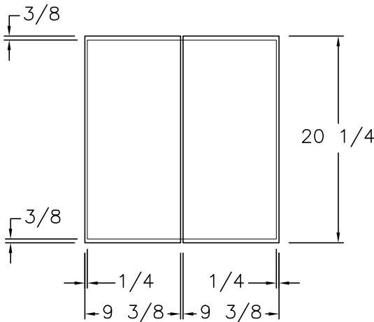
(4) 9 3/8 x 20 1/4 DOORS
