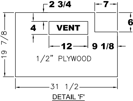
DETAIL 'F'
