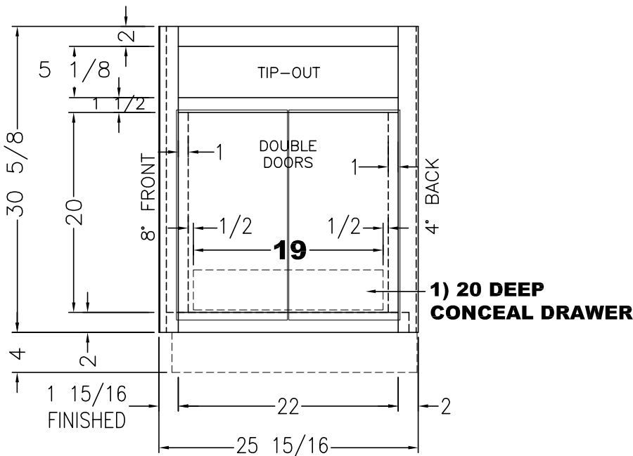
VIEW (E) (2) 11 1/8x20 3/4 DOORS (OVERSIZED @ BOTTOM) (1) 5 3/4x22 1/2 FRONT
