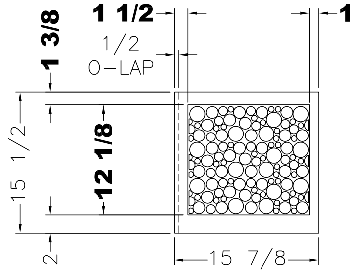
VIEW (B)
