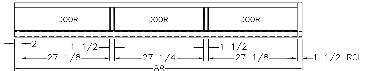
FRONT VIEW (3) 27 3/4 x 7 1/2 DOORS (TOP HG)
