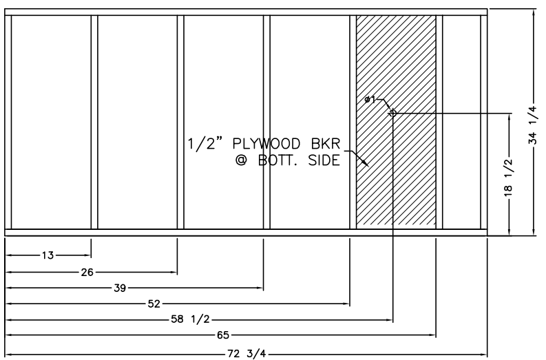
UPPER BUNK FRAME TOP VIEW
