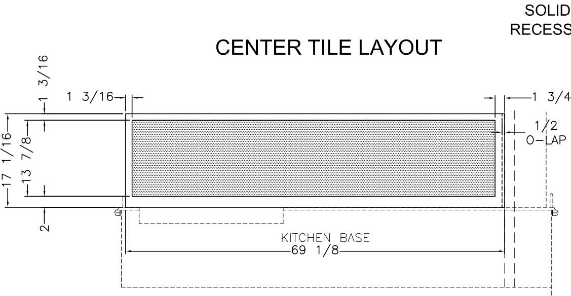
INSTALLATION DETAIL (SCALE 4X)
