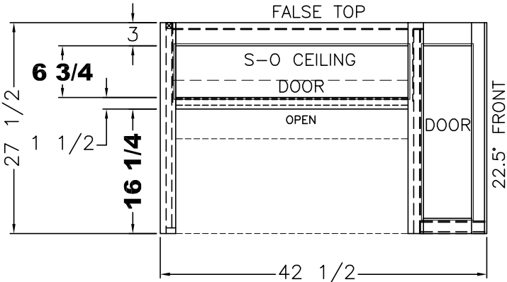
VIEW (B) (1) 7 1/4x30 3/4 HINGE DOOR (1) 6 3/4x23 1/4 DOOR
