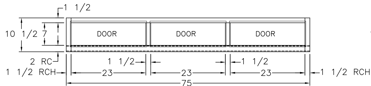
FRONT VIEW (3) 23 1/2 x 7 1/2 DOORS (TOP HG)
