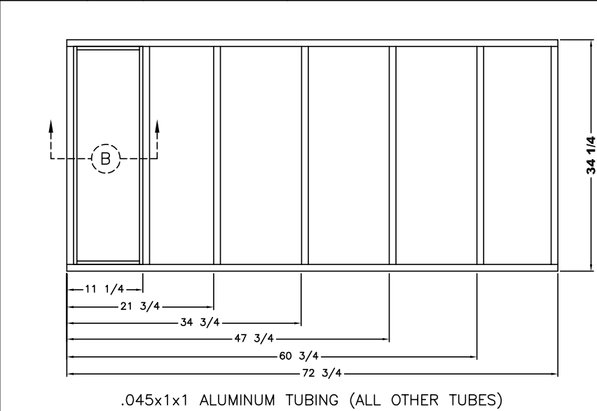
LOWER BUNK FRAME TOP VIEW
