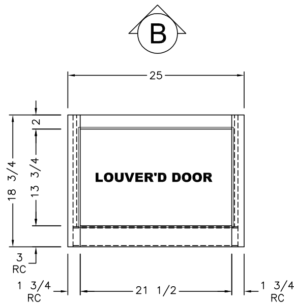
FRONT VIEW VIEW B
