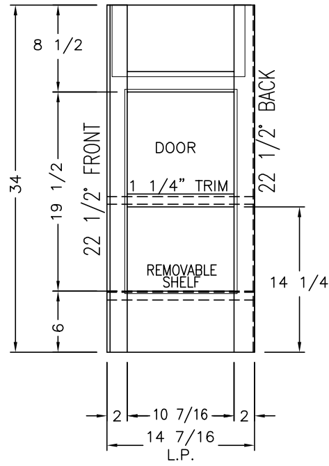
VIEW B
