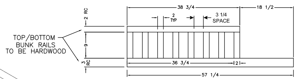
TOP BUNK RAILING
