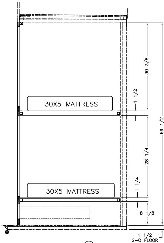
SECTION (A)
