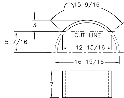
APRON DETAIL
