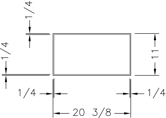
11x20 3/8 LOUV'D DOOR (BOTTOM HINGE)
