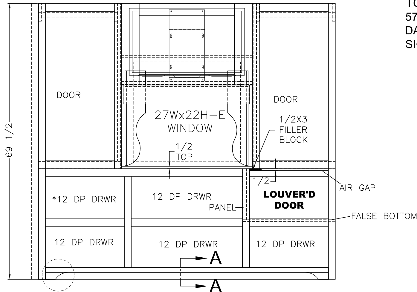
FRONT VIEW (1) 11x20 3/8 LOUVER'D DOOR (BOTTOM HINGE)
