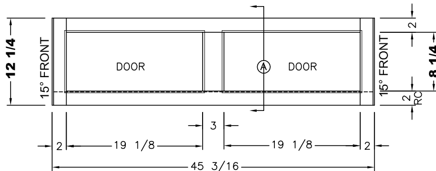
(2) 19 5/8x9 DOORS TOP HINGE
