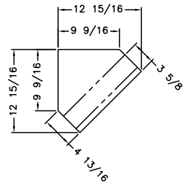
SHOWER TOP CORNER
