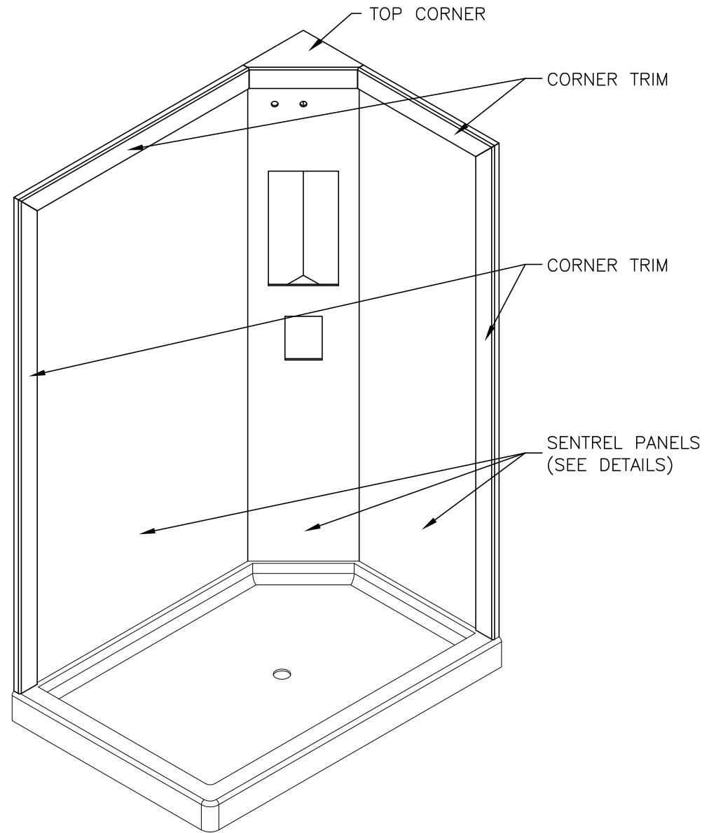
RIGHT HAND - ISO
