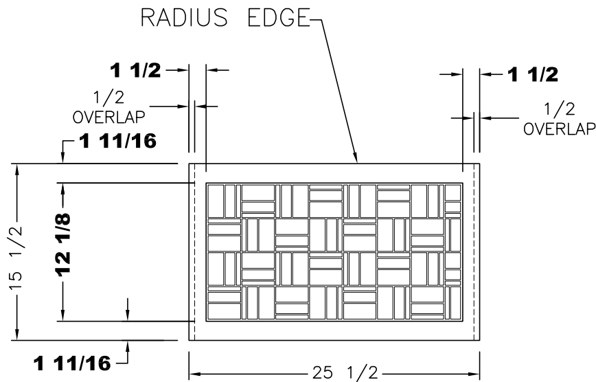
VIEW B
