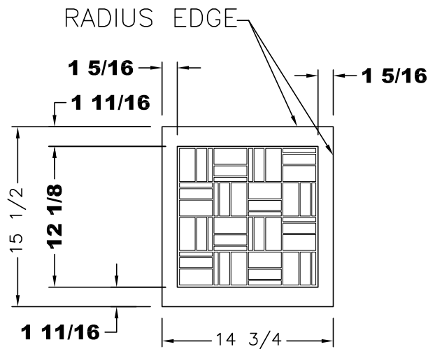
VIEW C
