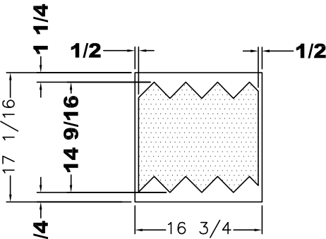
SIDE PANEL PIECE (ON WALL)
