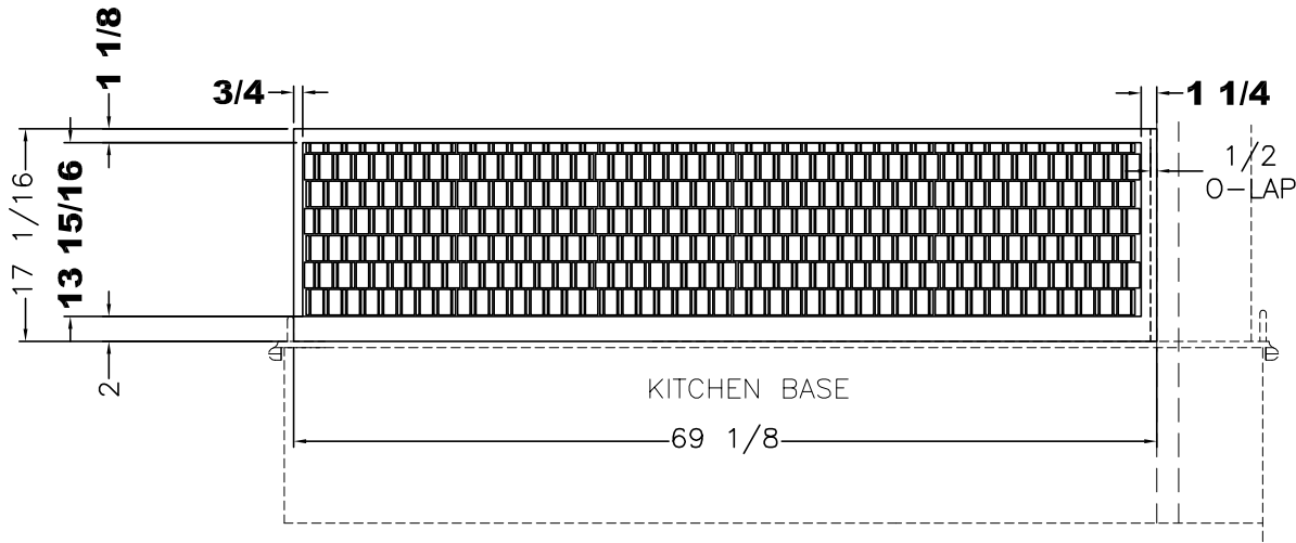
CENTER TILE LAYOUT
