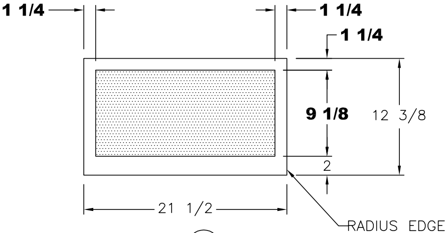
VIEW (C)
