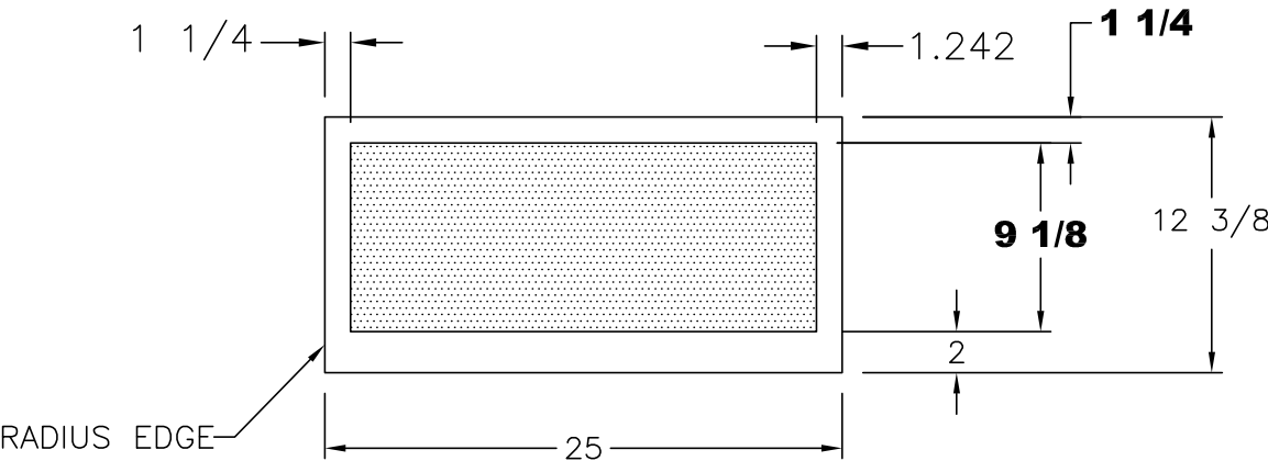
VIEW (A)
