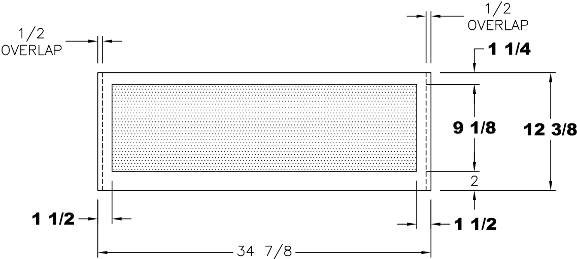
VIEW (B)
