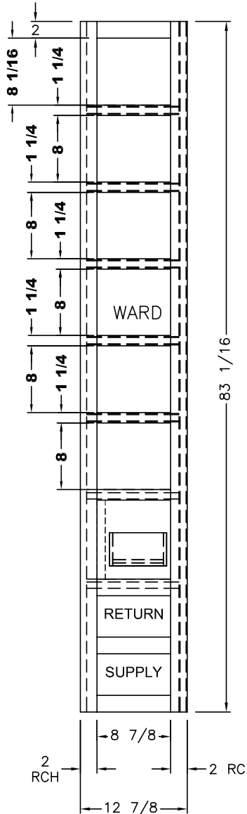
FRONT VIEW
