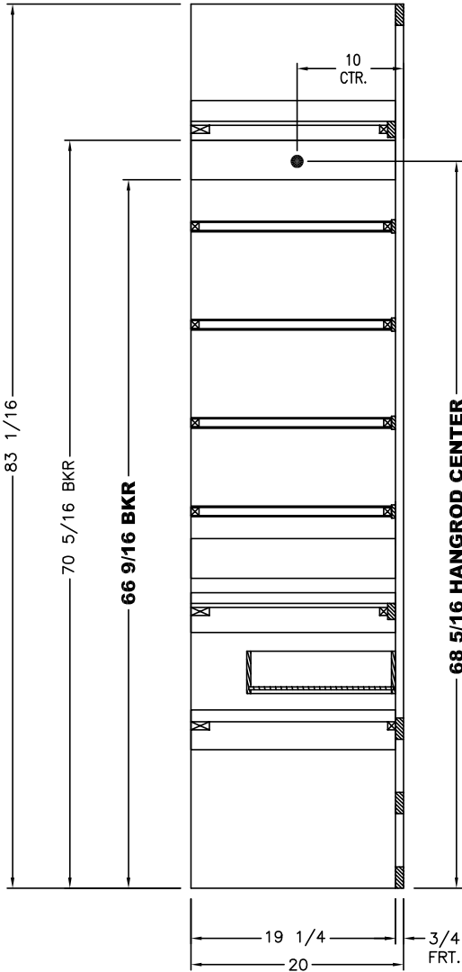
SECTION A
