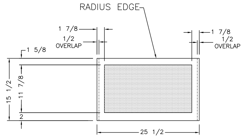
VIEW B
