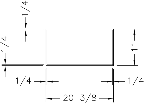
11x20 3/8 GLASS DOOR (BOTTOM HINGE)
