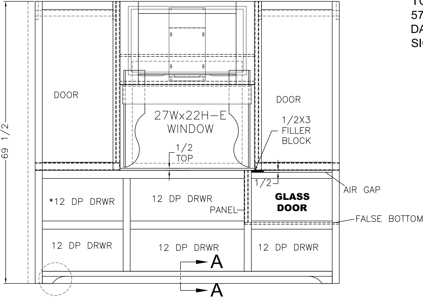
FRONT VIEW (1) 11x20 3/8 GLASS DOOR (BOTTOM HINGE)
