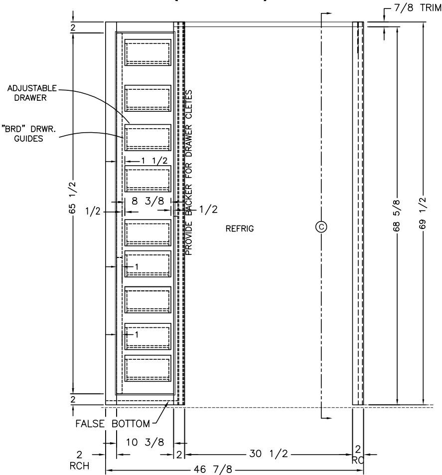
FRONT VIEW
