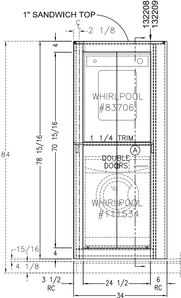
VIEW (A) (2) 12 3/8x71 1/2 LOUVERED DOORS
