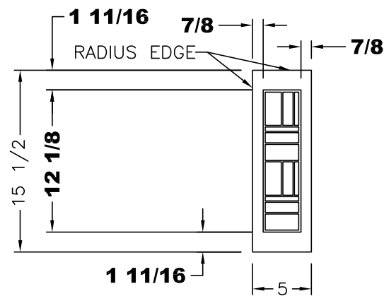
VIEW A
