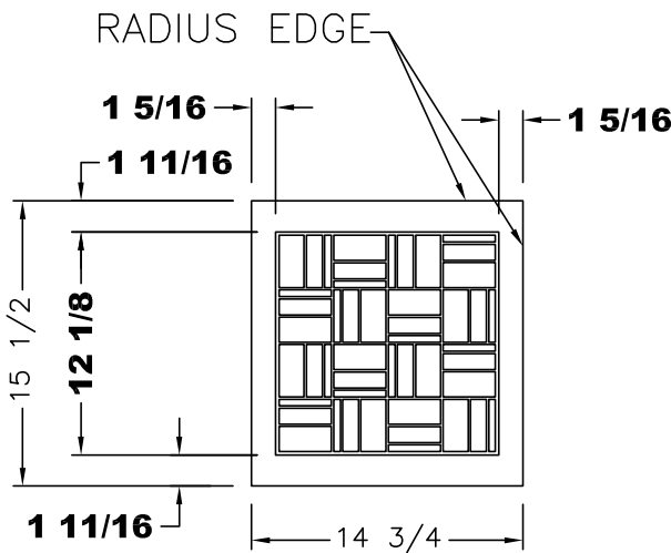
VIEW C
