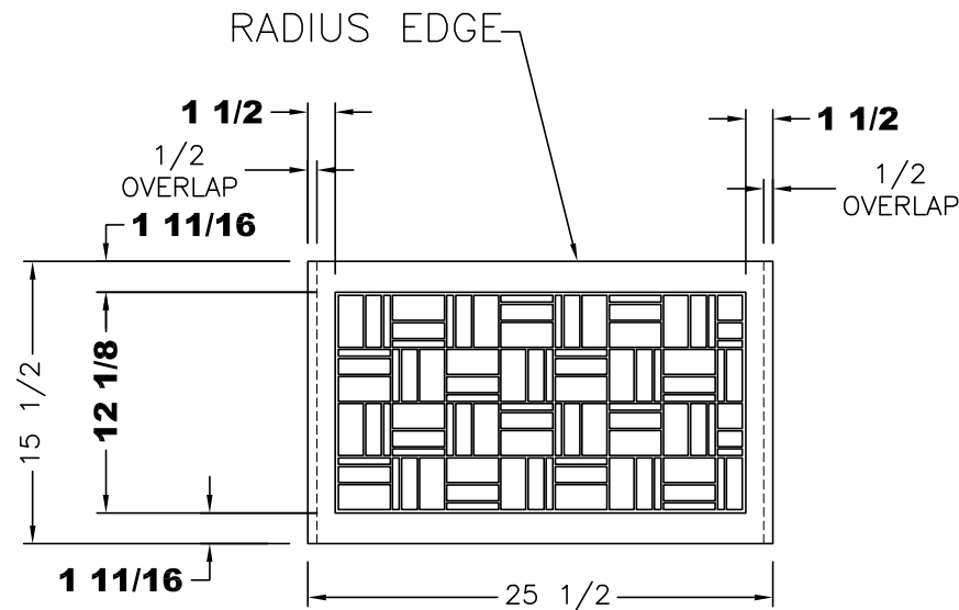
VIEW B
