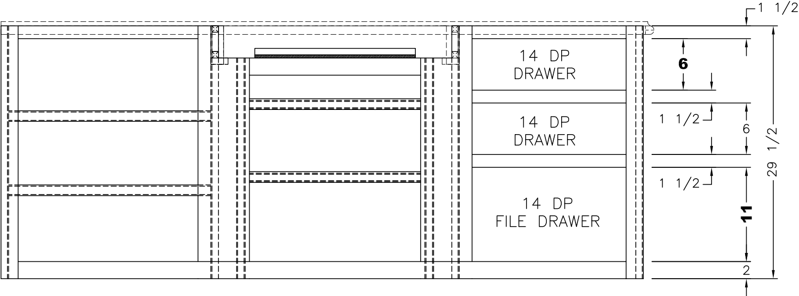
(2) 6 3/4x18 1/2 FRONT (1) 11 3/4x18 1/2 FRONT
