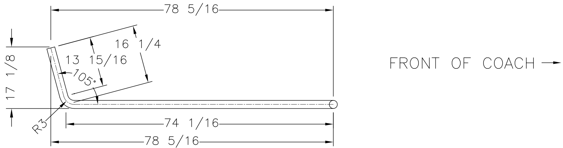
TOP VIEW
