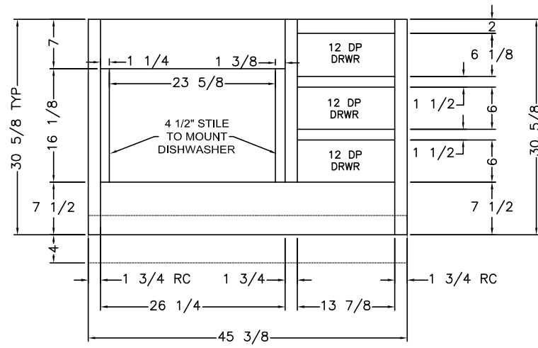
VIEW (A) (3) 6 5/8x14 3/8 FRONTS
