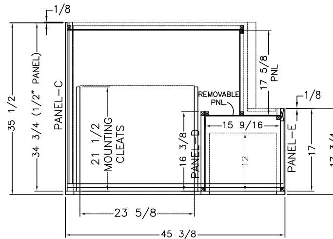
PLAN VIEW (A)
