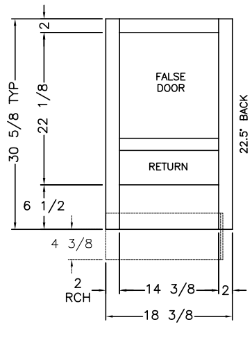
VIEW (B) (1) 14 7/8x15 7/8 FALSE DOOR
