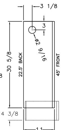
VIEW (E)
