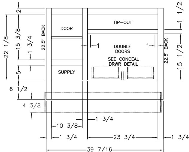
VIEW (C) (1) 10 7/8x15 7/8 DOOR (2) 12x16 DOORS (1) 5 5/8x24 1/4 DOOR
