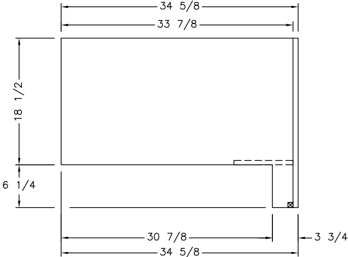
RT SIDE VIEW
