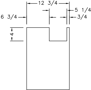
CHEST TOP 1/2" SOLID SURFACE ► — DENOTES A FINISHED EDGE
