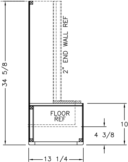
REAR CHEST TOP VIEW
