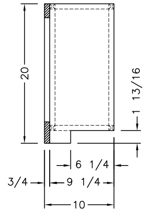
SIDE SECTION A
