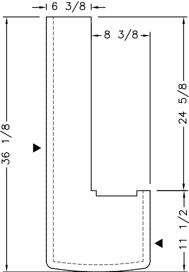
CHEST TOP 1/2" SOLID SURFACE ► — DENOTES A FINISHED EDGE
