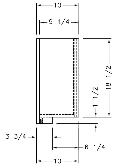
RT SIDE VIEW
