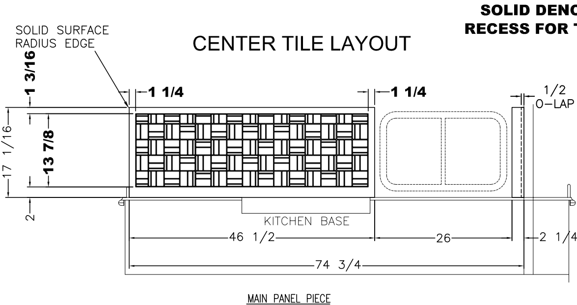
TILE/SOLID SURFACE BACKSPLASH (T360) KITCHEN WINDOW
