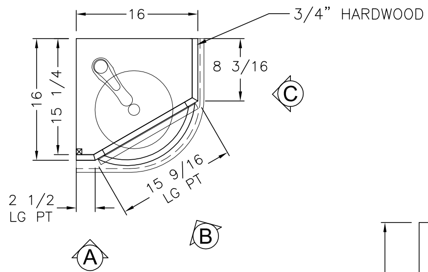
LAV. BASE (TOP VIEW)
