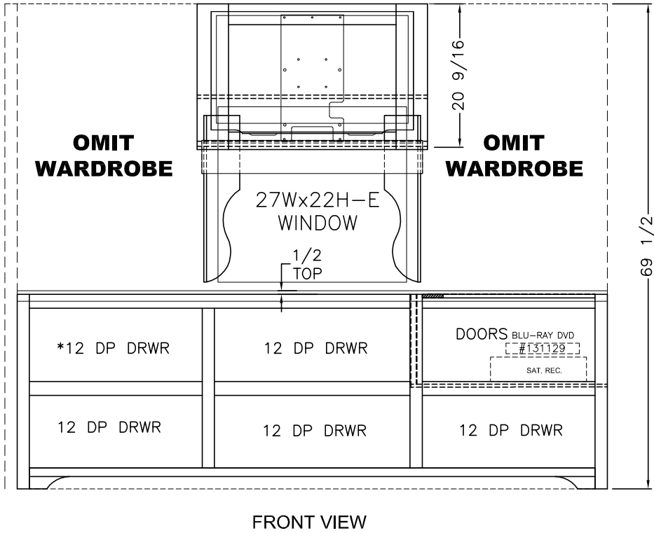
PLAN/DRESSER FRONT/SECTION
