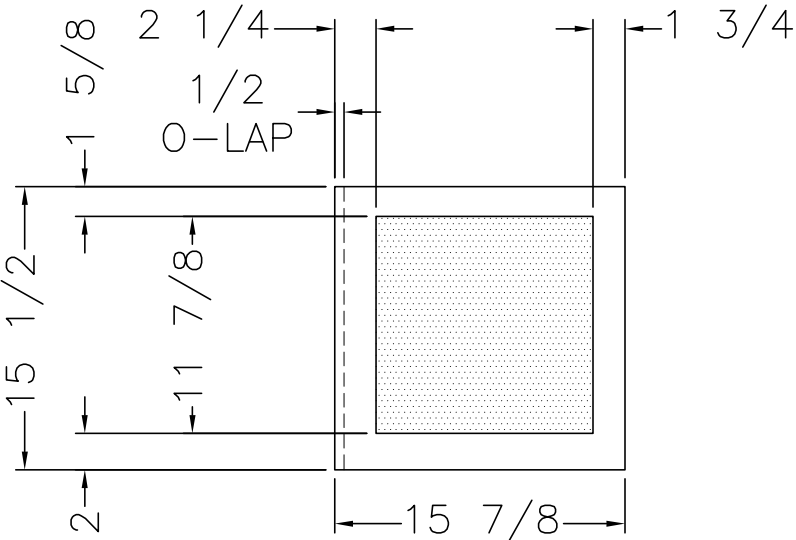
VIEW B
