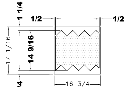
SIDE PANEL PIECE (ON WALL)
