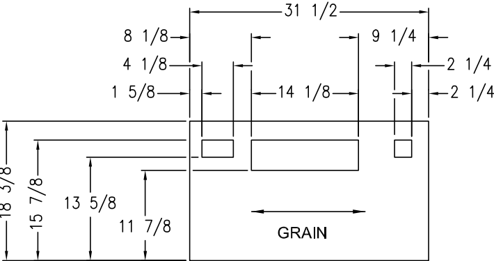
1/2 PLYWOOD DETAIL
