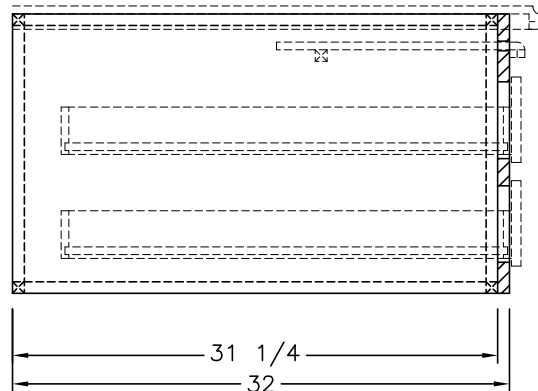
SIDE SECTION (A)
