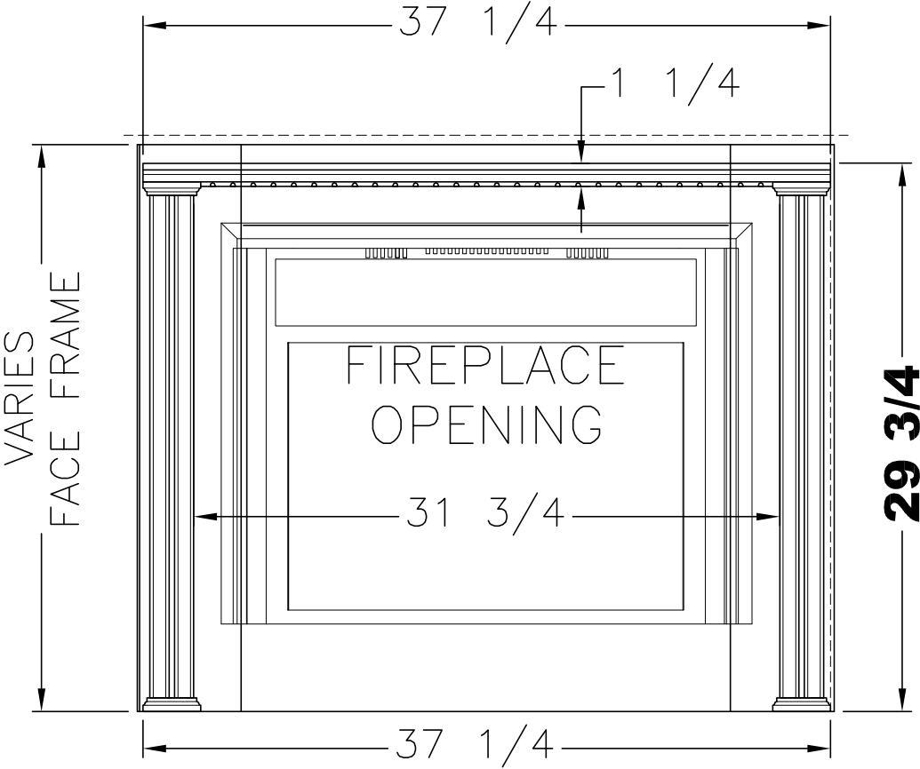
FRONT VIEW (ASSEMBLED)
