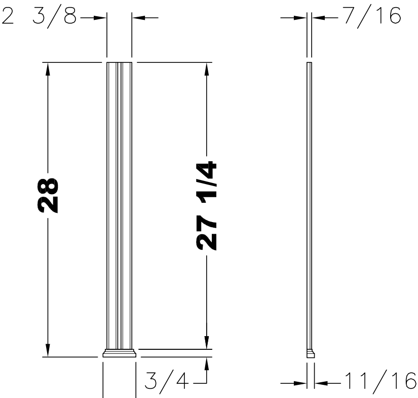
COLUMN DETAILS
