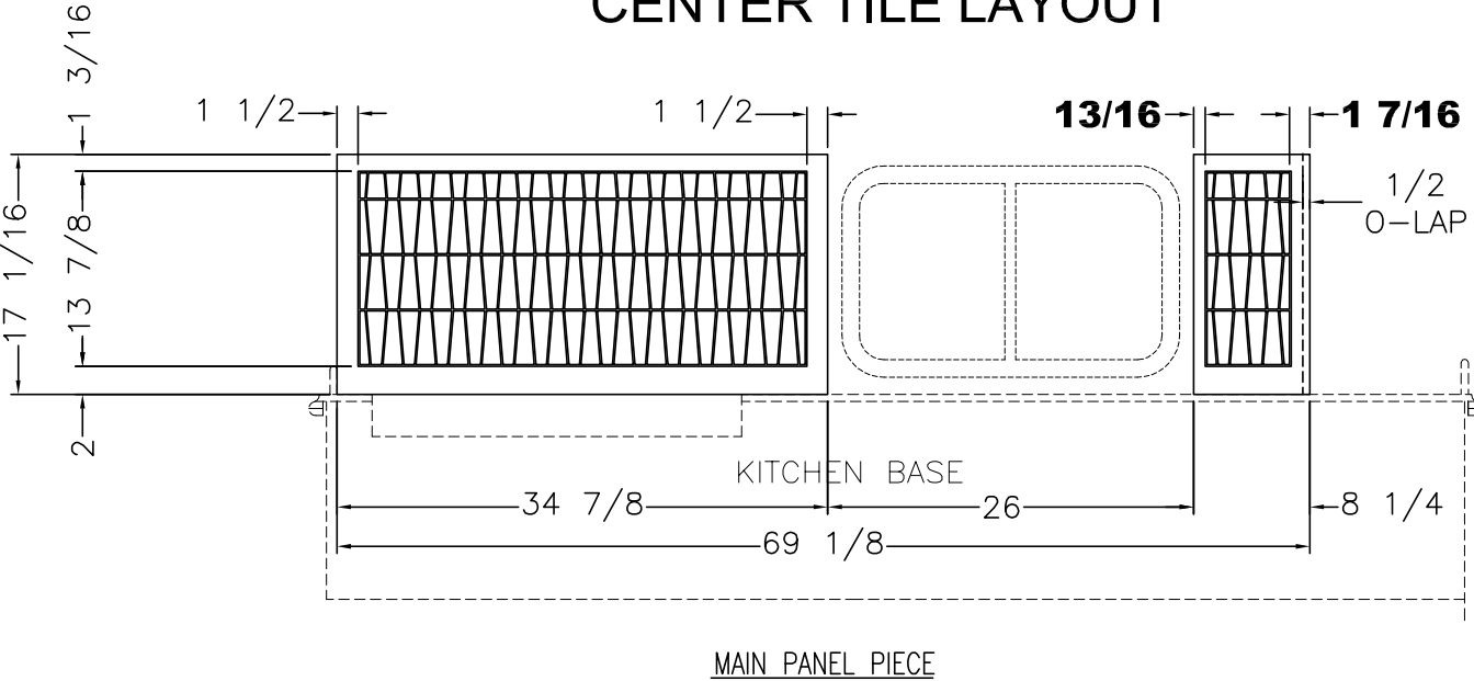
CENTER TILE LAYOUT
