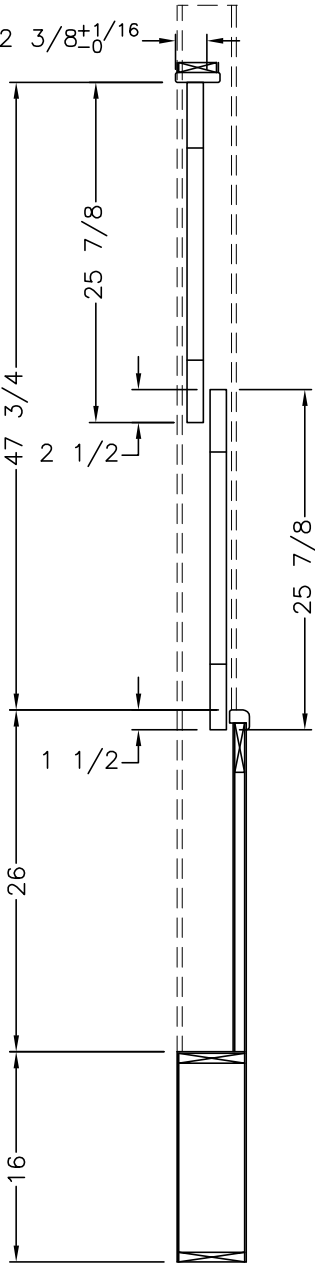
PLAN VIEW
