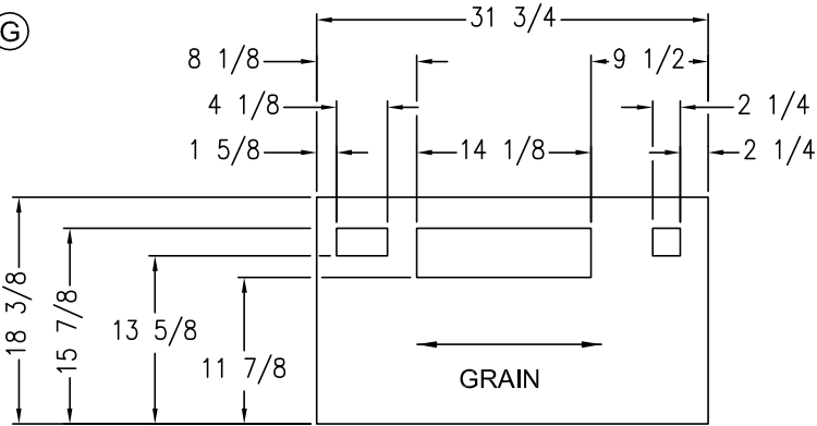
1/2 PLYWOOD DETAIL
