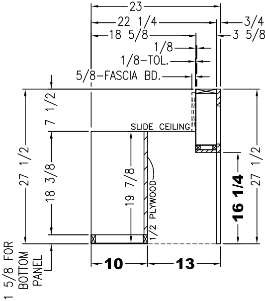
SIDE SECTION (G)
