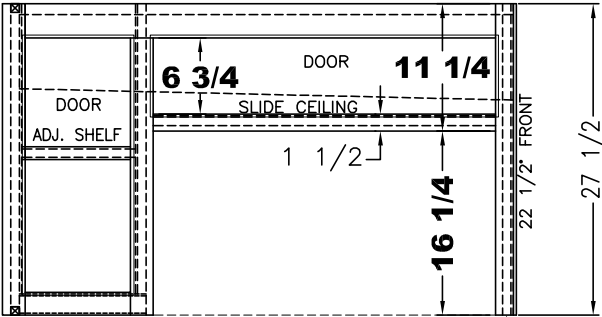
VIEW (B) (1) 7 1/4x30 3/4 HINGE DOOR (1) 9 7/8x23 DOOR
