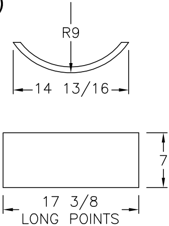
FRONT COVER LAID OUT FLAT
