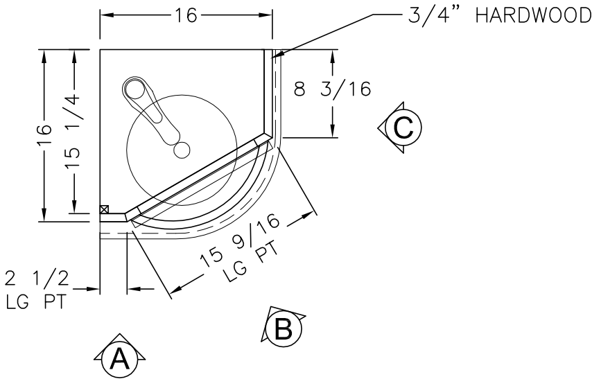
LAV. BASE (TOP VIEW)
