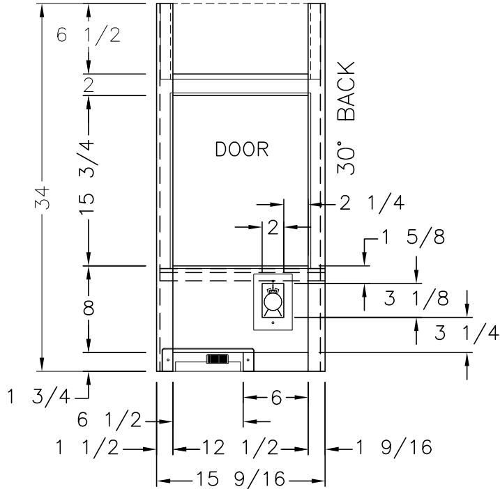
VIEW (B)
