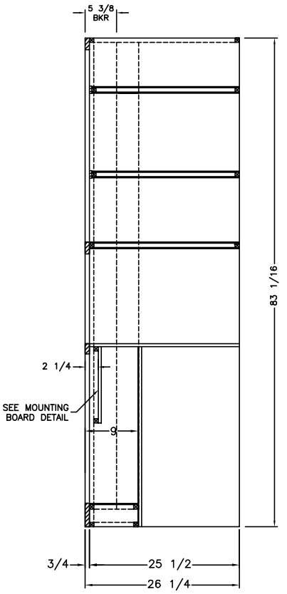
SIDE SECTION A
