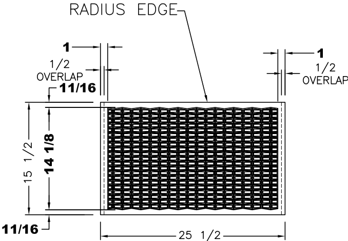
VIEW B
