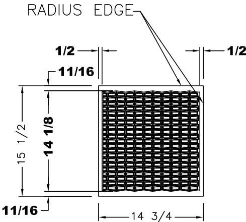
VIEW C
