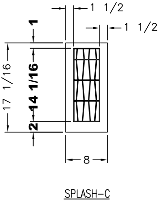
INSTALLATION DETAIL (SCALE 4X)
