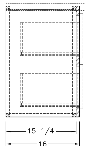
SIDE SECTION (A)
