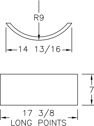
FRONT COVER LAID OUT FLAT
