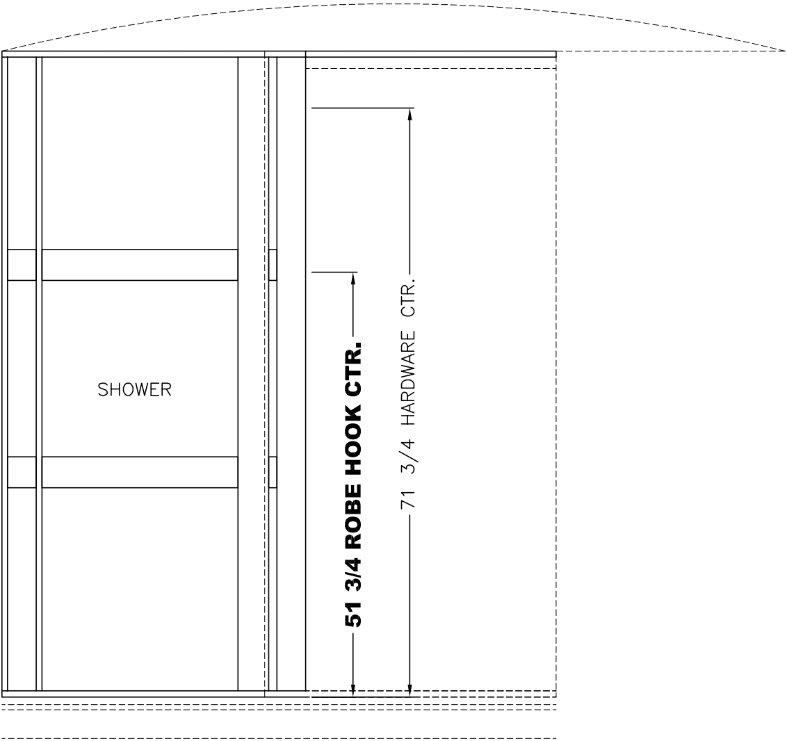
VIEW (A)
