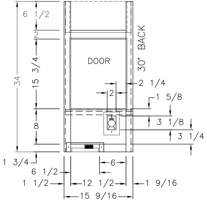
VIEW (B)
