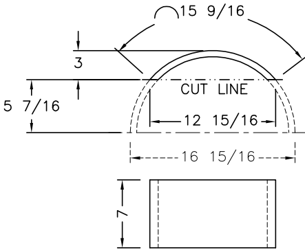
APRON DETAIL
