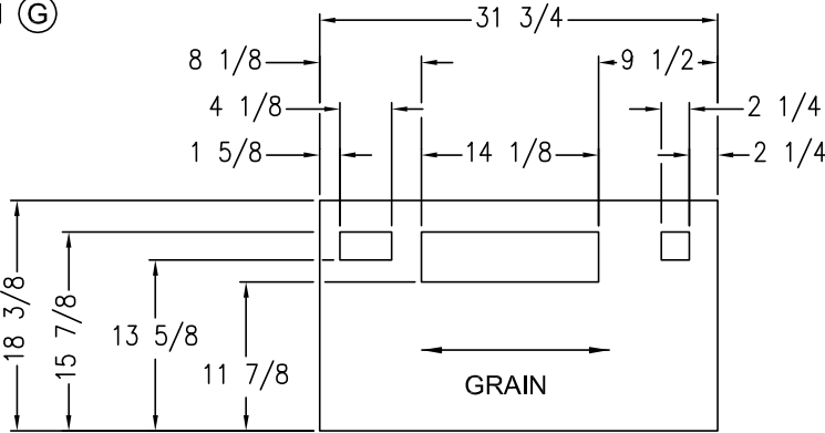
1/2 PLYWOOD DETAIL
